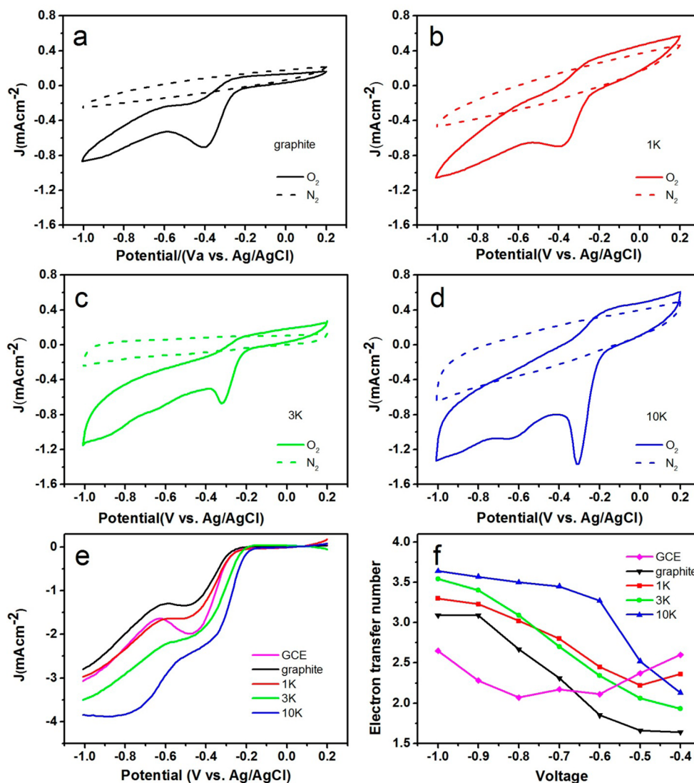
Figure 4. Cyclic voltammograms of catalysts in oxygen or nitrogen saturated 0.1 M KOH at a scan rate of 100 \text{ mV s}^{-1} . (a) Pristine graphite. (b) 1K. (c) 3K. (d) 10K. (e) Linear sweep performance at a rotation speed of 1600 rpm of the four catalysts in oxygen saturated 0.1 M KOH at a scan rate of 10 \text{ mV s}^{-1} . (f) Electrons transferred per oxygen molecule for the four catalysts over potential range -0.4 \text{ V} to -1.0 \text{ V} based on the Koutecky–Levich equation. For all electrochemical measurements, a 3 mm diameter BASI GCE was used and a catalyst loading of 0.283 \text{ mg/cm}^2 .
