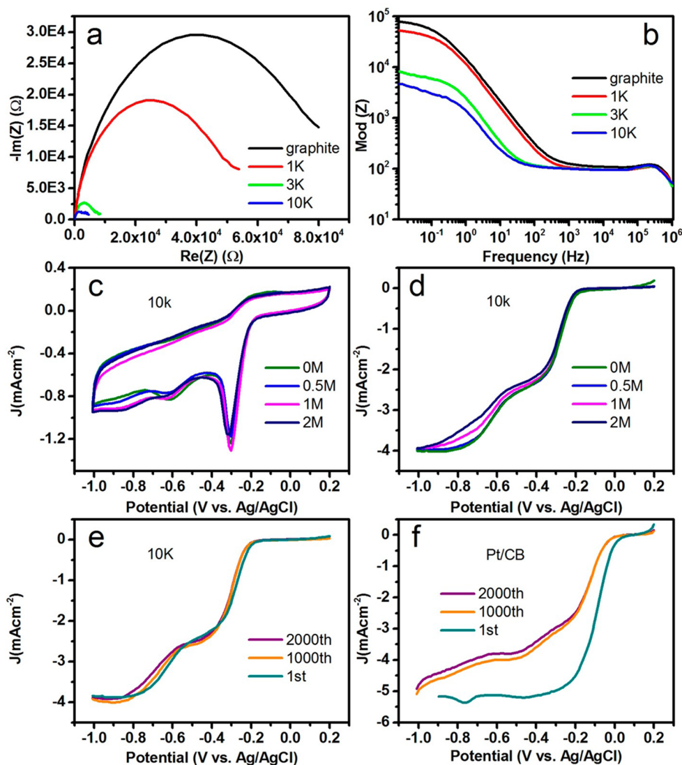
Figure 5. Electrochemical impedance spectroscopy plots in the form of (a) Nyquist and (b) Bode plots of the four catalysts. Measurements were performed at -0.2 V. (c) CV, (d) LS response of 10K nanosheets after methanol addition. (e) LS curves of 10K, (f) benchmark Pt/CB (20 wt % Pt) after 1st, 1000th, and 2000th CV scans. All measurements were carried out in oxygen saturated 0.1 M KOH using a 3 mm diameter BASI GCE and a catalyst loading of 0.283 \text{ mg/cm}^2 .
