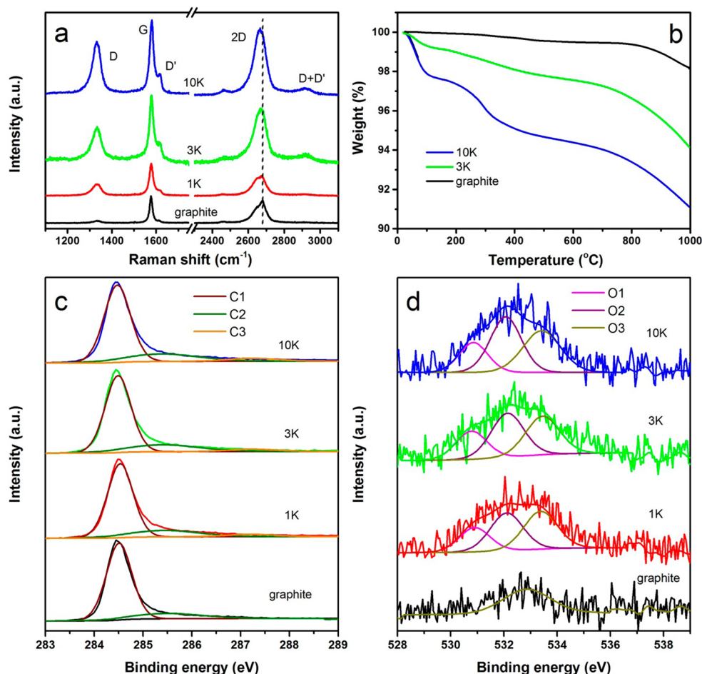
Figure 3. (a) Raman spectra showing increased D band intensity and a 2D peak downshift with increased symmetry indicating exfoliation and flake size reduction. (b) Thermogravimetric analysis (TGA) plots of graphite, 3K and 10K. Measurements were carried out under N 2 atmosphere with a heating rate of 5 °C min over the temperature range 24–1000 °C. High resolution (c) C 1s and (d) O 1s deconvoluted X-ray photoelectron spectroscopy (XPS) of graphite, 1K, 3K, and 10K.
